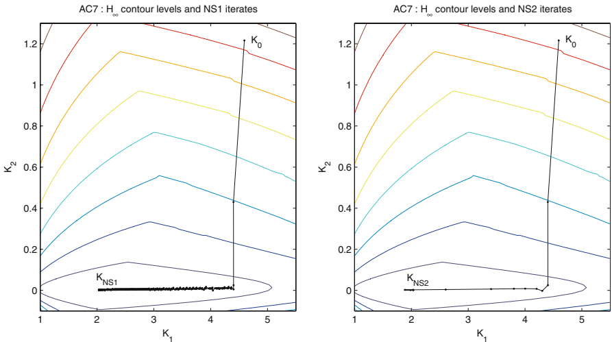
Fig. 2 Iterates in controller space for NS1 (left) and NS2 (right). NS2 is significantly faster despite the change of peaks caused by the non-smoothness
