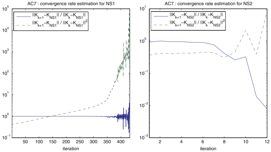
Fig. 1 Convergence rates of NS1 and NS2 for AC7. NS1 shows linear convergence with rate close to 1 (left). NS2 gives quadratic convergence (right)
